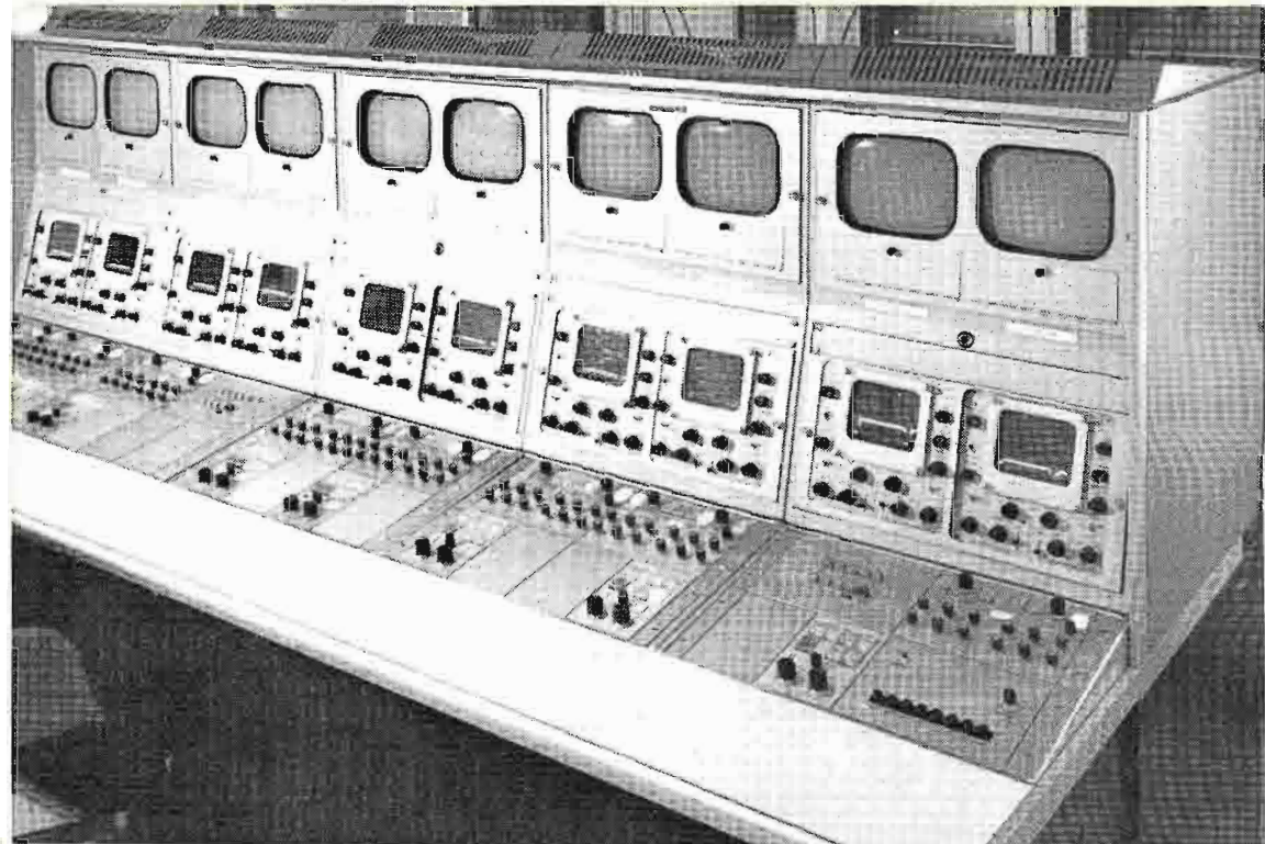
FIG. 15 Live camera control for eight color cameras; with studio output monitors, and two color camera match-monitor switchers.
