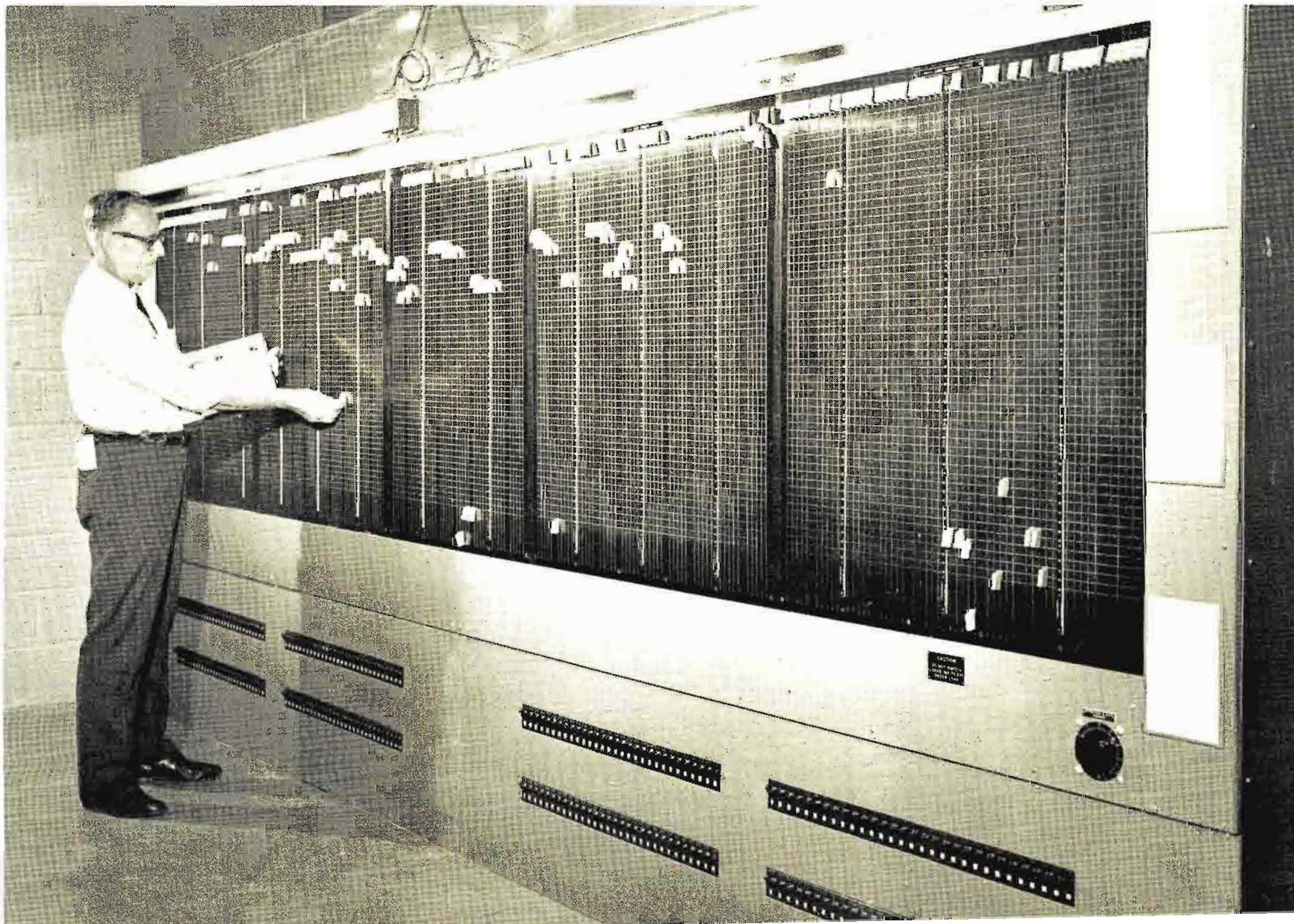
FIG. 8 Studio lighting panel—240 outlets on the lighting grid can be tied to any of forty 12KW dimmers or 15 "hot" circuits.
