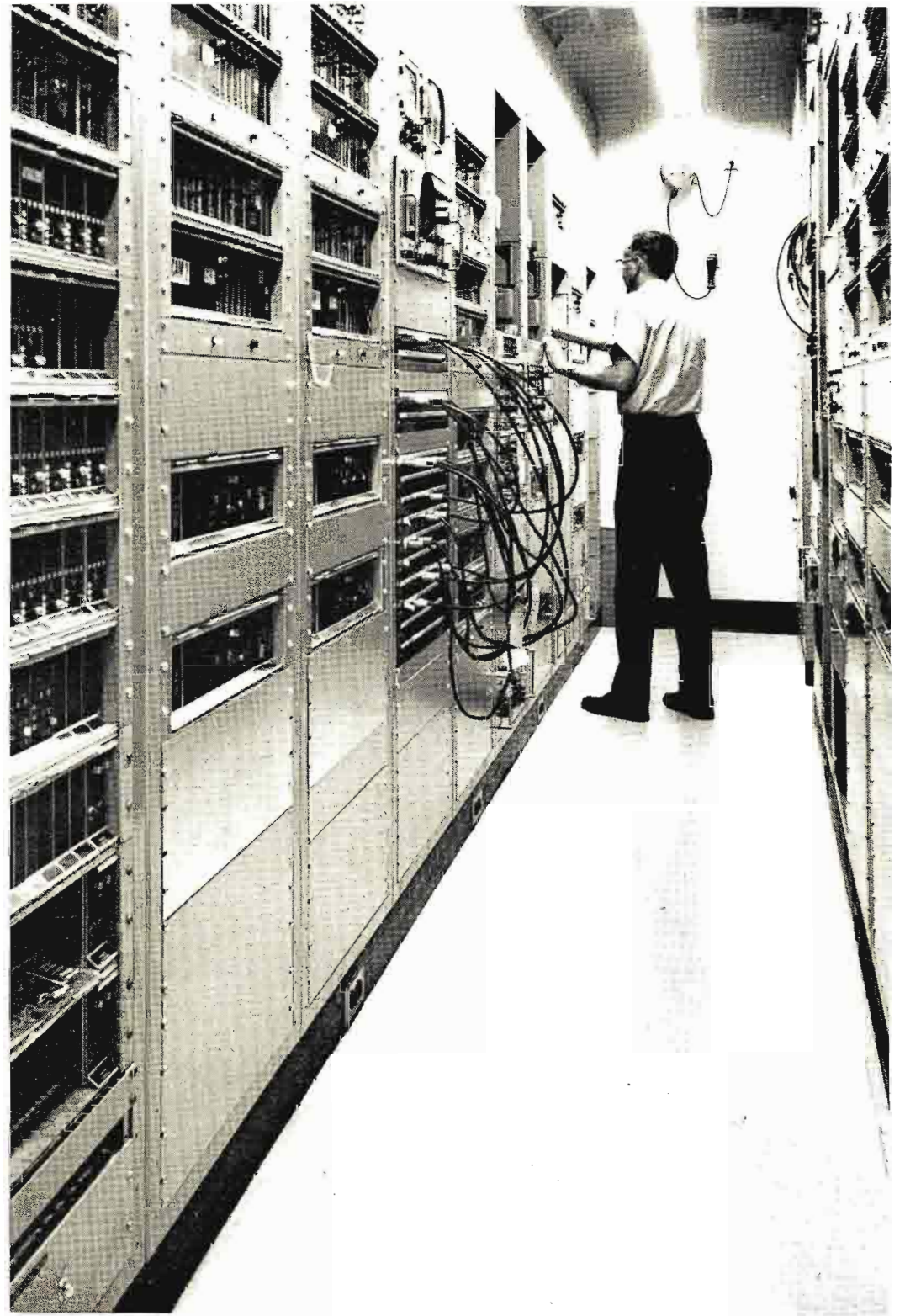
FIG. 17 Centralized electronics—an area for all rack-mounted equipment, which speeds servicing and reduces video runs.
