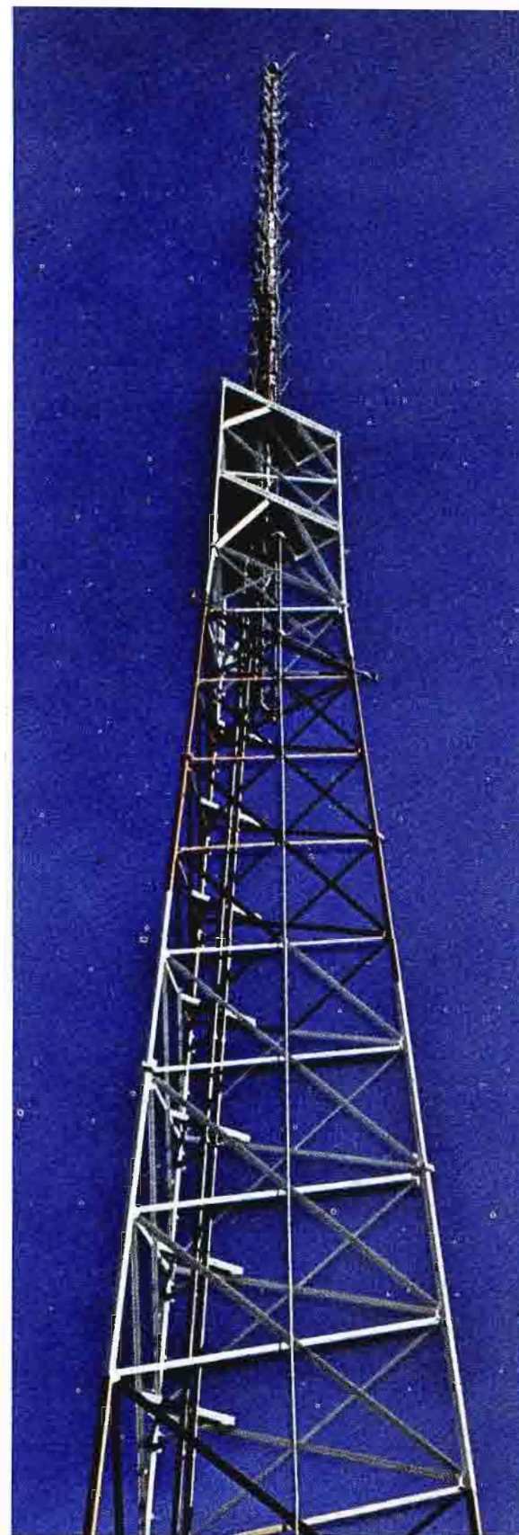
FIG. 15 The TF-12AH superturnstile antenna tops the 100-foot tower on Black Mountain—1220 feet above average terrain. This is also the site of KHBV, the Channel 5 commercial station.
